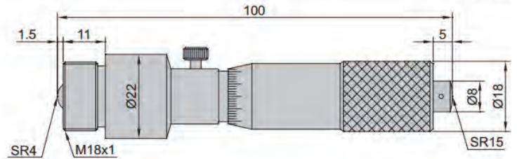
IM-9022 Micrometer head
