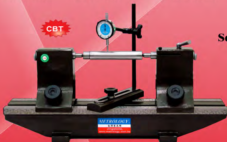
Concentricity Test Bench
